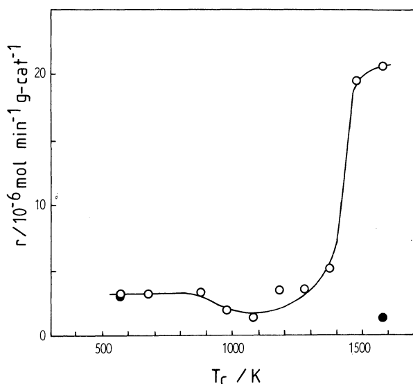
Fig. 2. Dependence of the reaction rate, r , of cobalt sulfide catalyst for the hydrogenation of butadiene at 473 K upon the calcination temperature T_c of the precursor cobalt oxide. Both sulfidation and H_2 -treatment temperatures were 673 K. O; after H_2 treatment and ●; before H_2 treatment.
