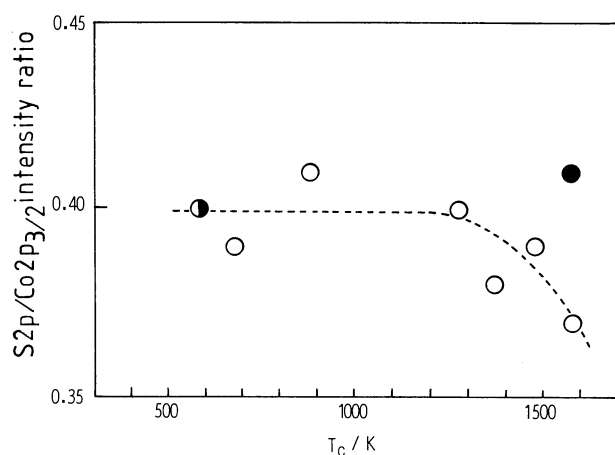
Fig. 5. Dependence of the S2p/Co2p 3/2 XPS intensity ratio for cobalt sulfide catalysts upon T_c . Both sulfidation and H_2 -treatment temperatures were 673 K. ○; after H_2 -treatment and ●; before H_2 -treatment. The ratios were averaged over 2–5 independent measurements.
